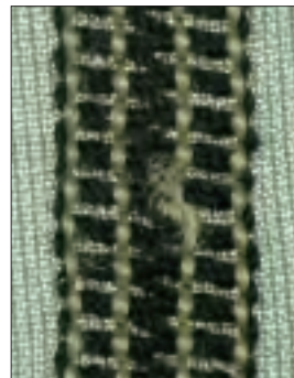
Missed thread pick up using woolly thread
